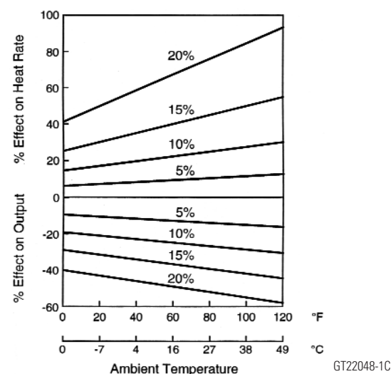
Figure 15. Effect of air extraction on output and heat rate
