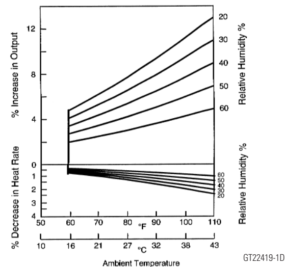
Figure 16. Effect of evaporative cooling on output and heat rate
