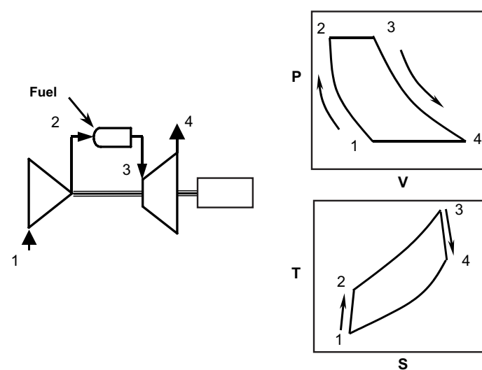
Figure 4. Brayton cycle
