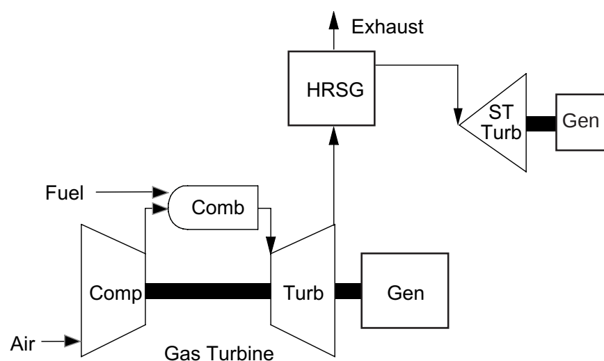
Figure 8. Combined cycle
