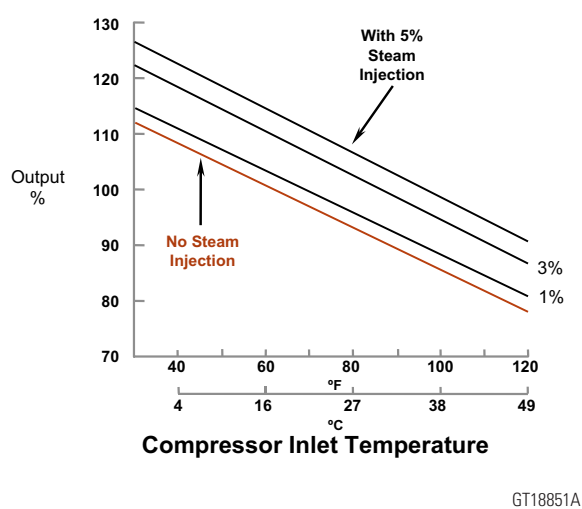
Figure 14. Effect of steam injection on output and heat rate
