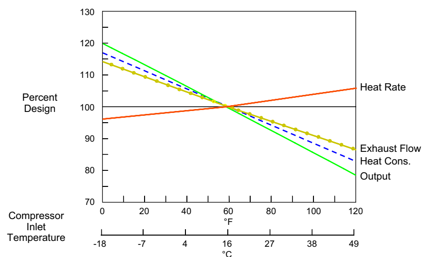
Figure 9. Effect of ambient temperature
