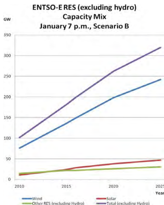
Figure 3.2.23: ENTSO-E Renewable Energy Sources installed capacity mix
