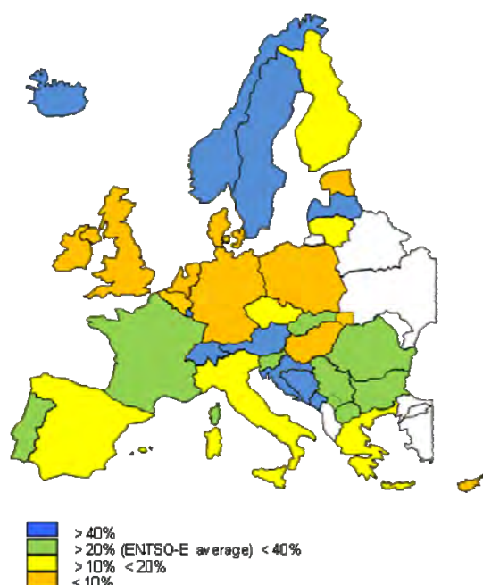
Figure 3.2.18: Share of Hydro power units in NGC per country in January 2015, 7 p.m., Scenario B
