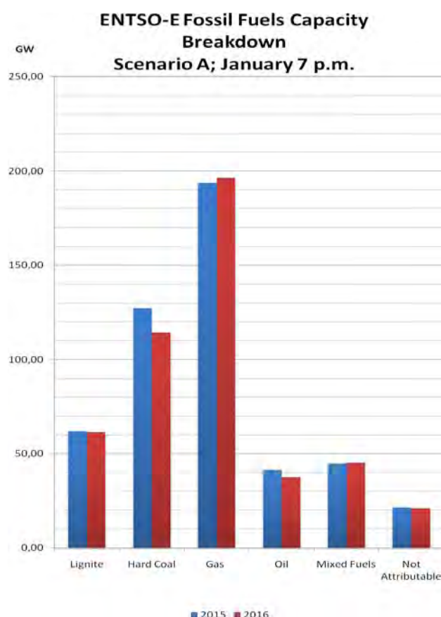
Figure 3.2.10: ENTSO-E Fossil Fuels Capacity Breakdown
