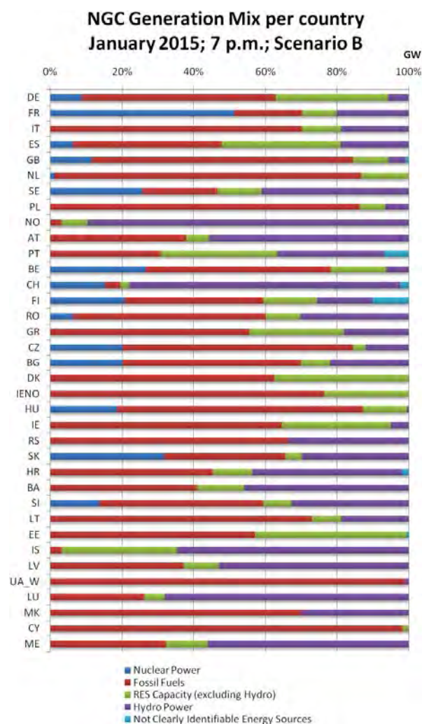
Figure 3.2.7: Net Generating Capacity Generation Mix
