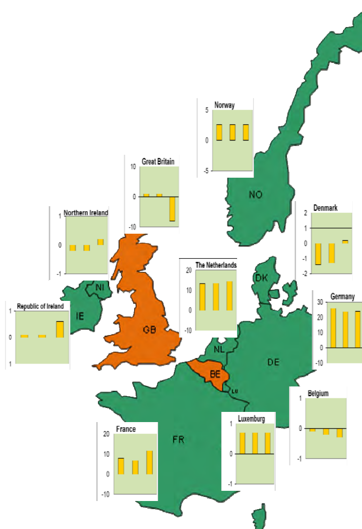
Figure 4.1.1: Remaining capacity minus Adequacy Reference Margin for each country in RG NS in 2020 (Scenario B)
